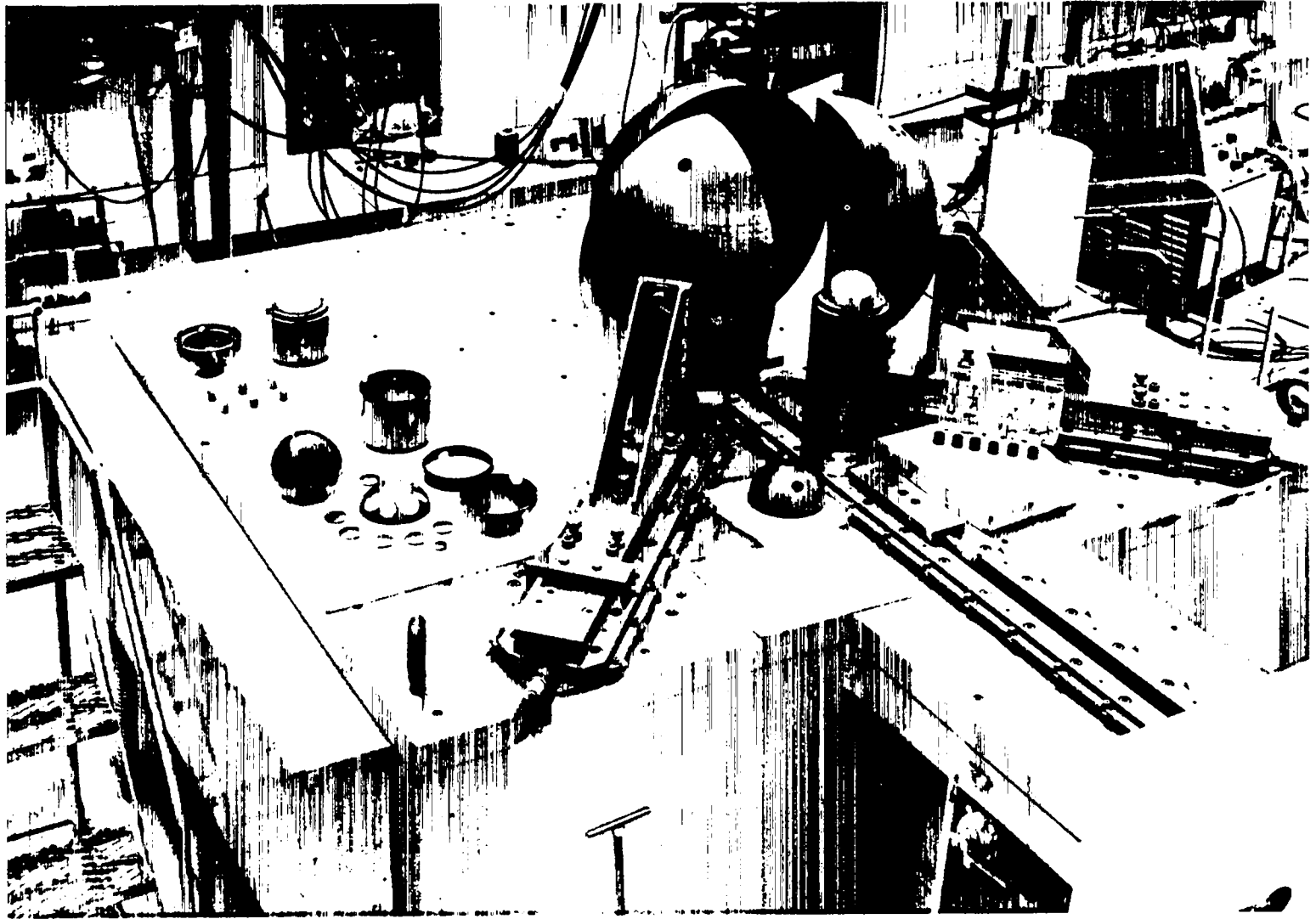
Fig. 20. The Flattop critical assembly machine. The plutonium core is shown retracted from the natural-uranium reflector; enriched-uranium and ^{233}\text{U} cores with adapters are laid out at left.
